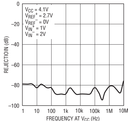
Power Supply Rejection vs Frequency at V_{CC}
