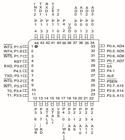
44-Pin QFP
