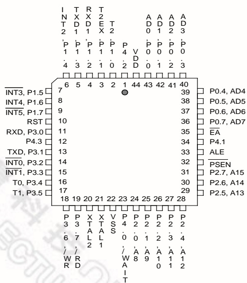
44-Pin PLCC
