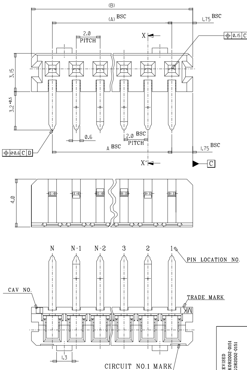
SECTION X-X' SCALE 10:1
