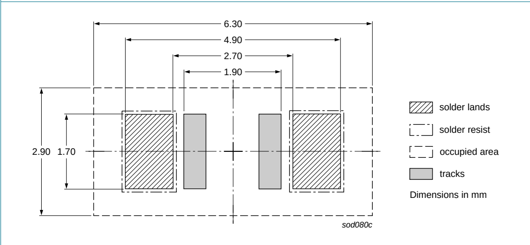
Fig 8. Wave soldering footprint SOD80C
