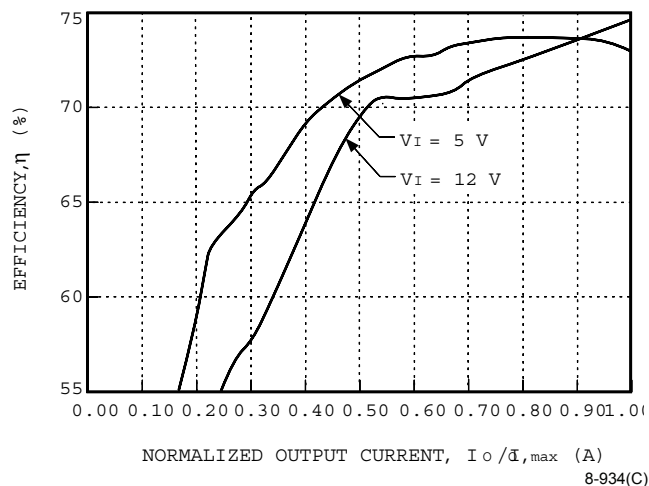
Figure 11. MH005B, C, BK, CL Typical Converter Efficiency as a Function of Output Current; T_A = 25 °C
