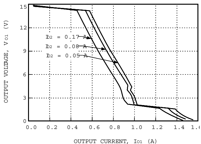
Figure 9. MH005CL Typical Output Characteristics with V_I = 12 V and T_A = 25 °C
