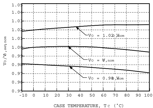
Figure 2. MH005-Series Typical Output Voltage Variation over Operating Case Temperature
