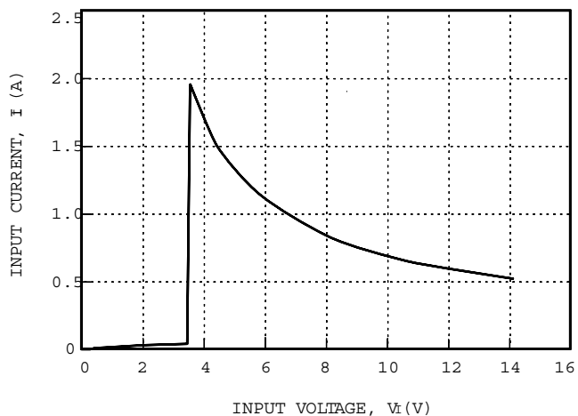
Figure 1. MH005-Series Typical Input Characteristics with I_o = I_{o, \max} and T_A = 25^\circ\text{C}
