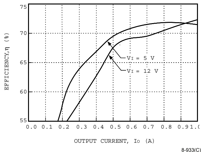
Figure 10. MH005A Typical Converter Efficiency as a Function of Output Current; T_A = 25 °C
