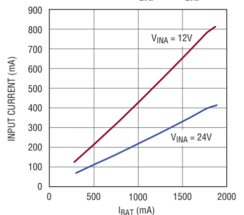
Input Current vs I_{BAT} , 4.2V BAT
