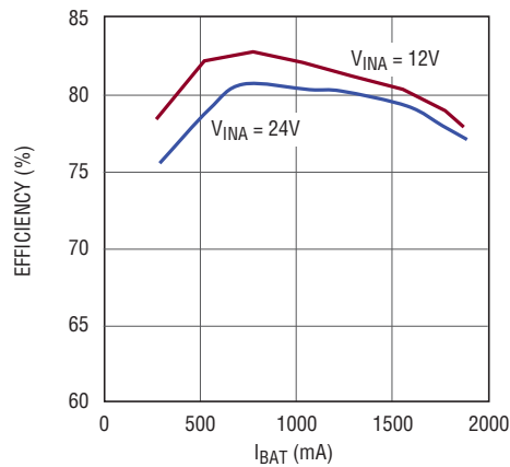
Efficiency vs I_{BAT} , 4.2V BAT
