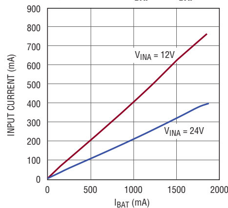
Input Current vs I_{BAT} , 4.1V BAT
