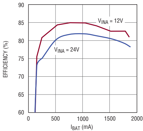
Efficiency vs I_{BAT} , 4.1V BAT
