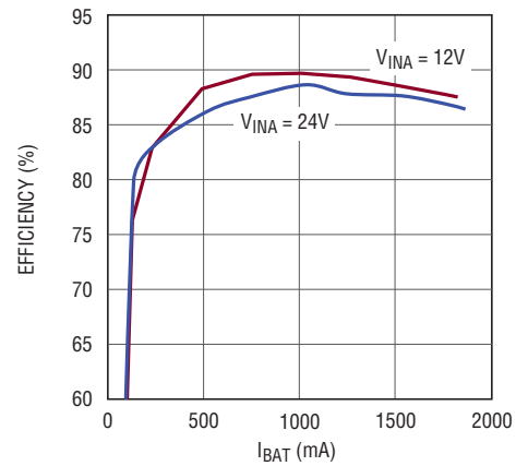
Efficiency vs I_{BAT} , 8.2V BAT
