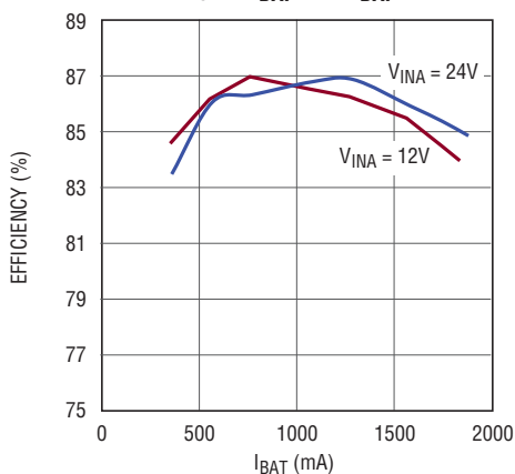
Efficiency vs I_{BAT} , 8.4V BAT
