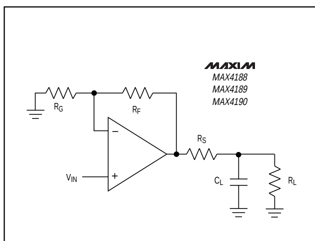
Figure 6a. Using an Isolation Resistor ( R_S ) for High Capacitive Loads
