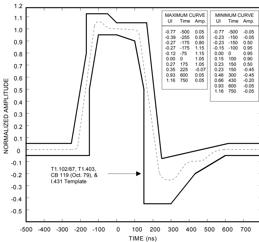
Figure 11-2. T1 Transmit Pulse Template
