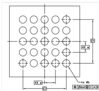
Figure 12. WLCSP (2.6x2.6x0.5) package outline
