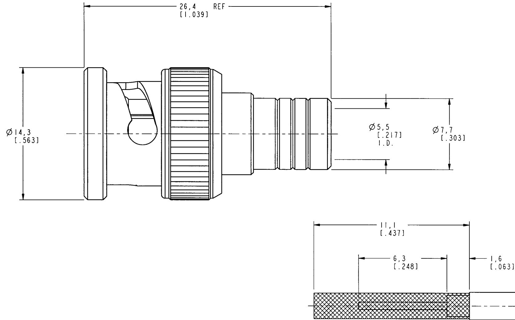
RECOMMENDED CABLE STRIPPING DIM'S. SCALE : 6.000
