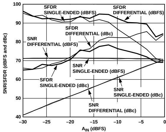
Figure 15. AD9235-65: Single Tone SNR/SFDR vs. A_{IN} with f_{IN} = \text{Nyquist} (32.5 MHz)
