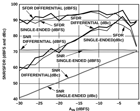
Figure 17. AD9235-20: Single Tone SNR/SFDR vs. A_{IN} with f_{IN} = \text{Nyquist} (10 MHz)
