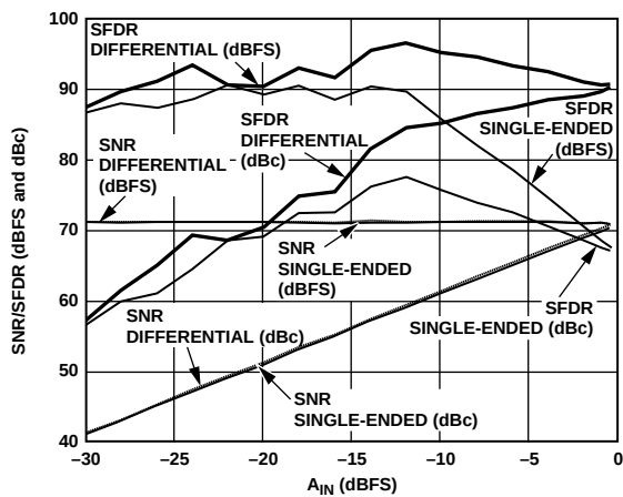
Figure 16. AD9235-40: Single Tone SNR/SFDR vs. A_{IN} with f_{IN} = \text{Nyquist} (20 MHz)
