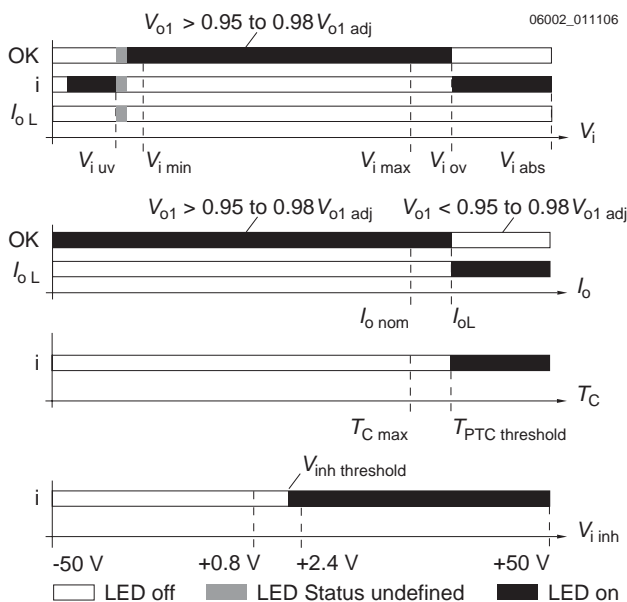
Fig. 23 LED indicators
