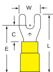
33-6-P Stud Size 6 Wire Range 12-10
