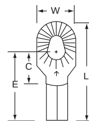
13-610 Stud Size 6, 8, 10 Wire Range 12-10
