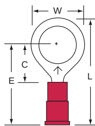
11-38-P Stud Size Wire Range 3/8 22-18
