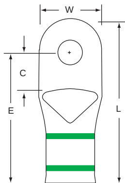
MC1-14RX Stud Size Wire Range 1/4 1
