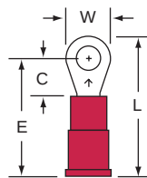
11-6S-P Stud Size Wire Range 6 22-18
