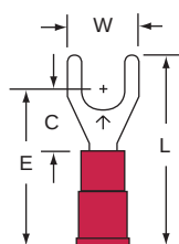
31-10-P Stud Size 10 Wire Range 22-18
