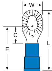
12-610-P Stud Size Wire Range
