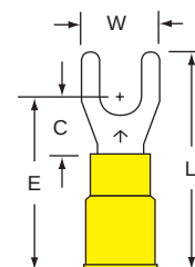
33-10-P Stud Size 10 Wire Range 12-10
