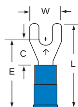
32-6-P Stud Size 6 Wire Range 16-14
