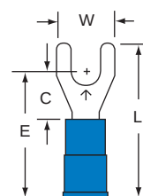
32-8-P Stud Size 8 Wire Range 16-14
