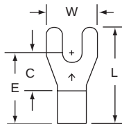
33-6-W Stud Size 6 Wire Range 12-10
