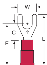
31-8-P Stud Size 8 Wire Range 22-18
