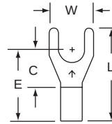
32-8-W Stud Size 8 Wire Range 16-14
