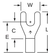
32-6-W Stud Size 6 Wire Range 16-14
