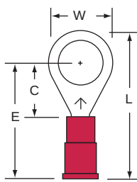
11-56S-P Stud Size Wire Range 5/16 22-18
