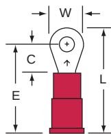
11-4S-P Stud Size Wire Range 4 22-18
