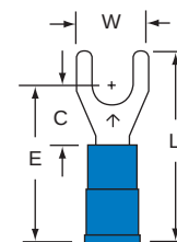
32-10-P Stud Size 10 Wire Range 16-14
