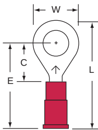
11-14S-P Stud Size Wire Range 1/4 22-18
