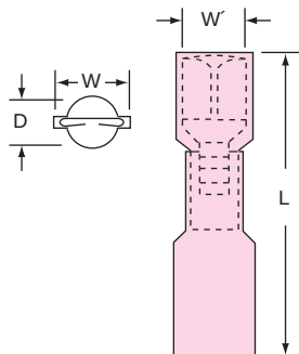
MNHU18-250DFI Wire Range 22-18
