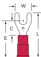
31-6-P Stud Size 6 Wire Range 22-18
