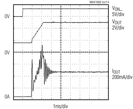
AUXILIARY CONTROLLER STARTUP RESPONSE
