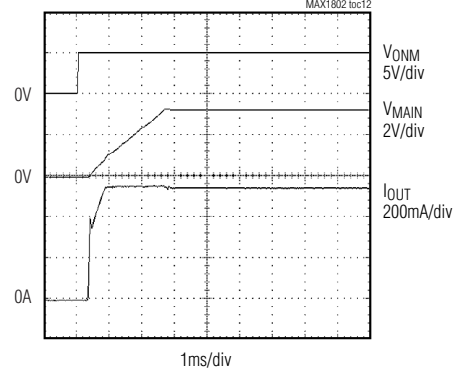
MAIN OUTPUT STARTUP RESPONSE
