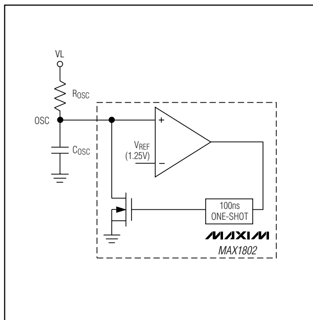
Figure 4. Oscillator
