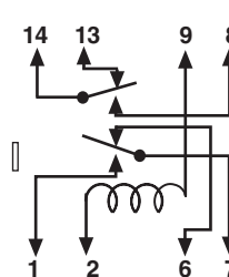
DPDT
