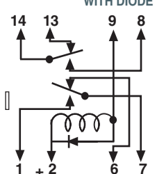
DPDT
