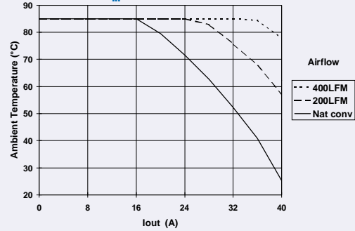
PT7761 @ V_{in} = 5V
