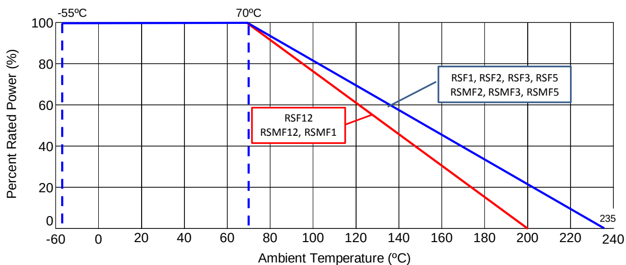
Power Derating Curve:
