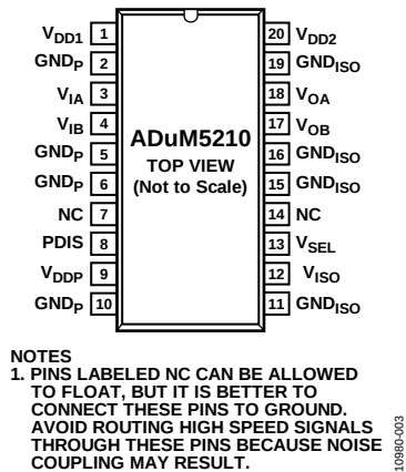
Figure 3. ADuM5210 Pin Configuration
