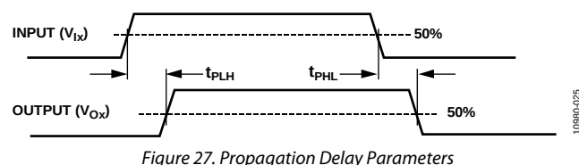
Figure 27. Propagation Delay Parameters
