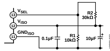
Figure 25. V_{ISO} Bias and Bypass Components
