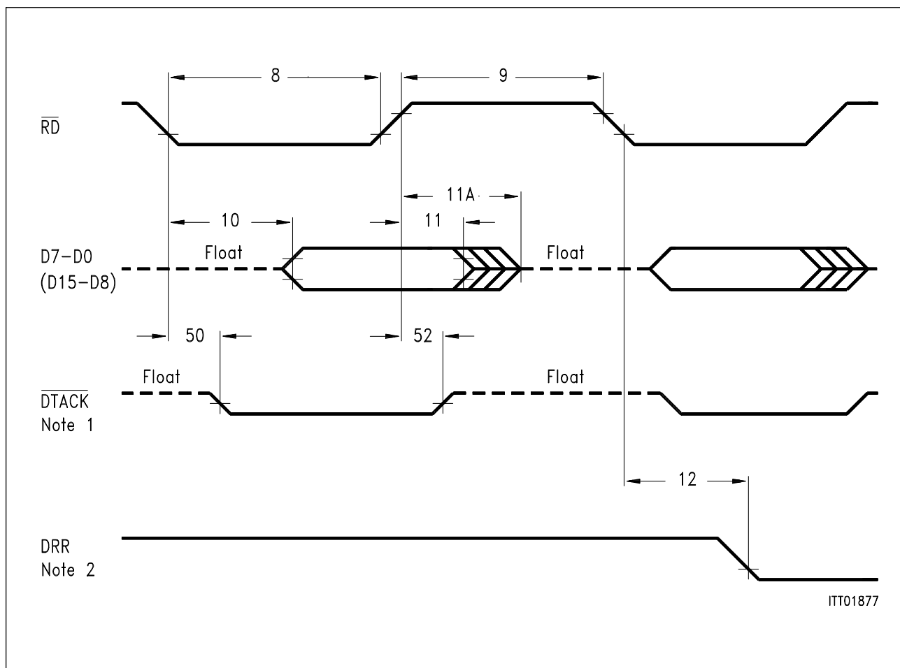
Figure 56 Siemens/Intel Read Cycle Timing
