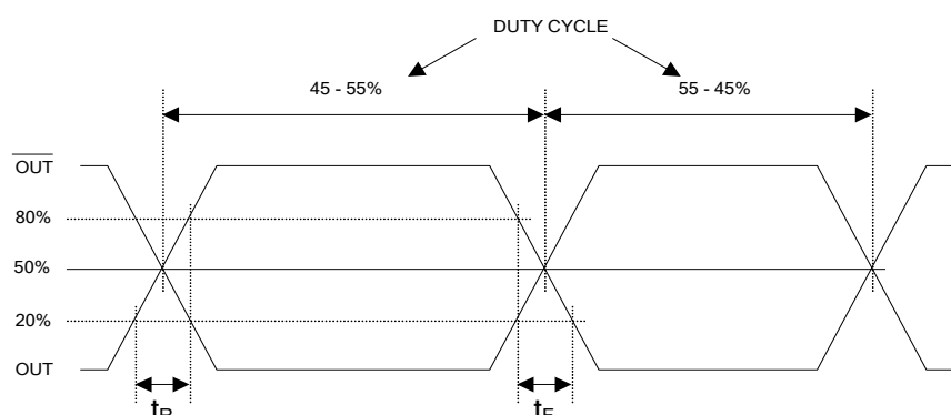
LVPECL Transistion Time Waveform
