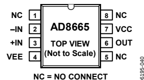
Figure 2. AD8665, 8-Lead SOIC_N (R-8)
