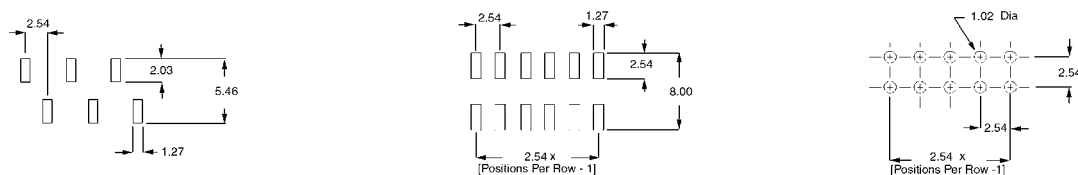
Recommended PCB layouts
