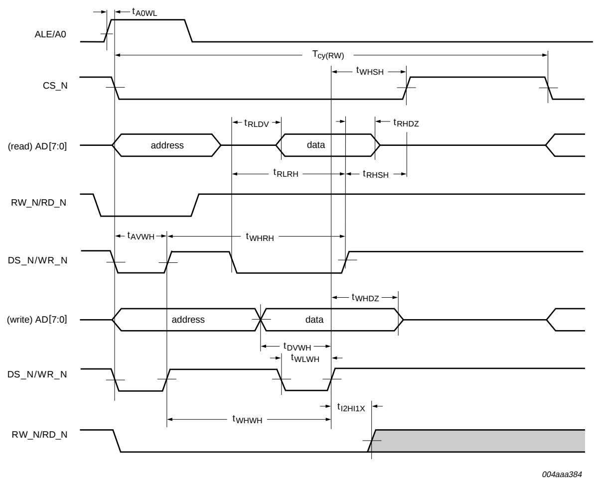
Fig 29. ISP1583 register access timing: multiplexed address/data bus (A0 function and Freescale mode)
