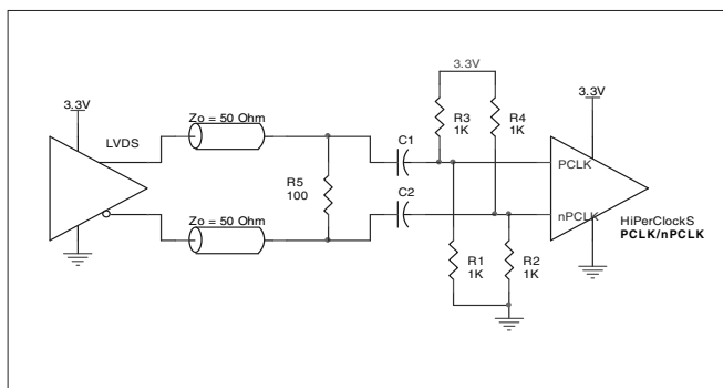
FIGURE 5F. PCLK/nPCLK INPUT DRIVEN BY A 3.3V LVDS DRIVER
