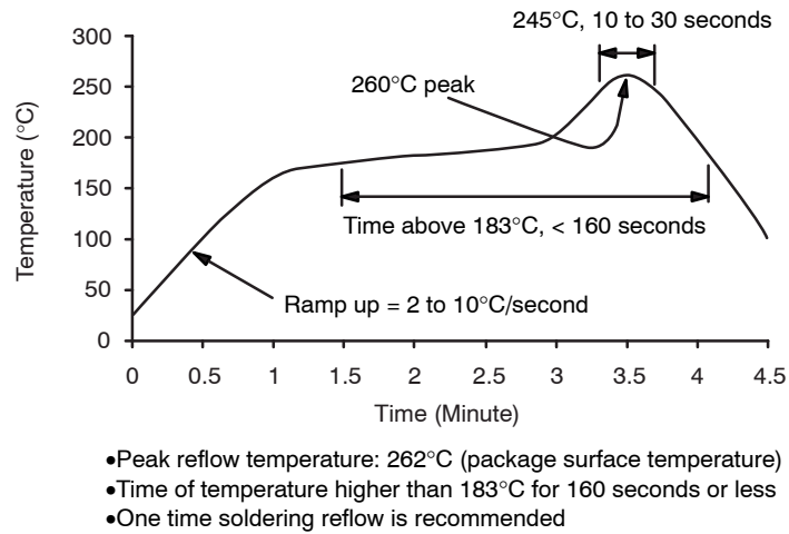
Figure 12. Reflow Profile
