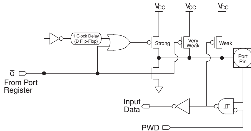
Figure 11-2. Quasi-bidirectional Output
