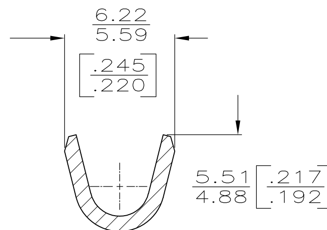
SECTION Y-Y
