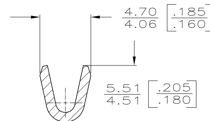
SECTION X-X
