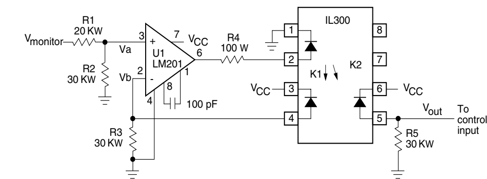
Figure 18. DC Coupled Power Supply Feedback Amplifier
