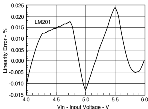
Figure 20. Linearity Error vs. Input Voltage
