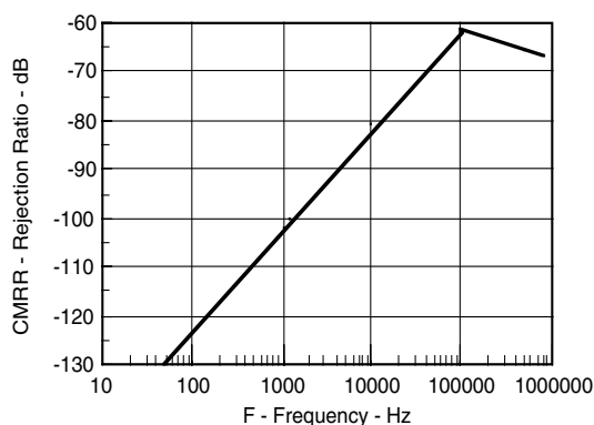
Figure 14. Common-Mode Rejection
