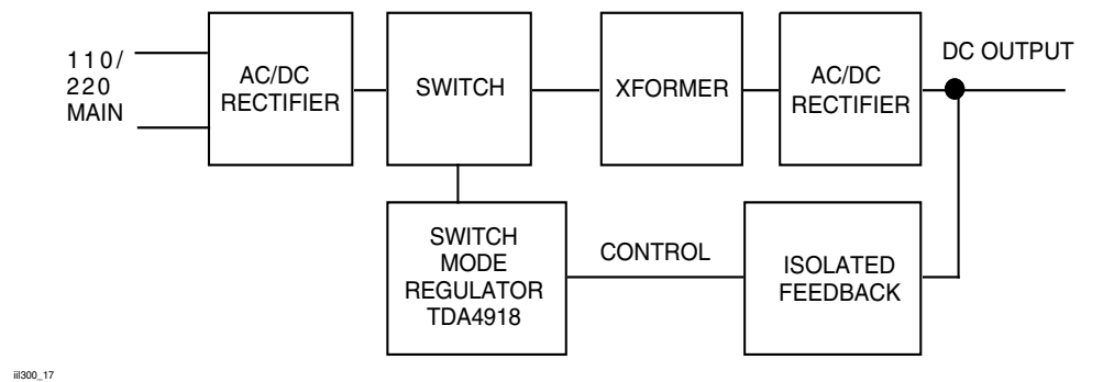
Figure 17. Switching Mode Power Supply
