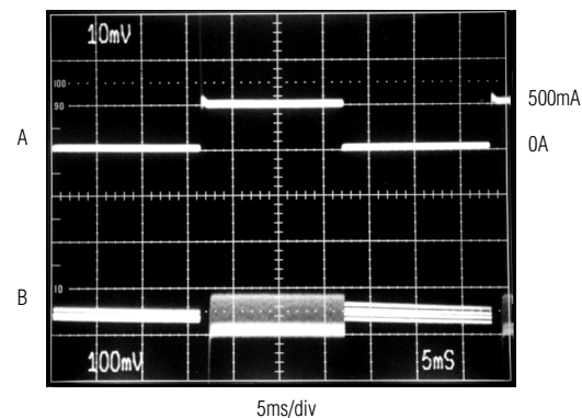
LOAD-TRANSIENT RESPONSE
