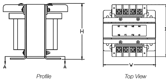
Mounting Dimensions
