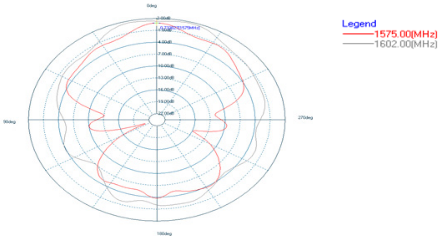
XZ Plane (PHI=0°)
