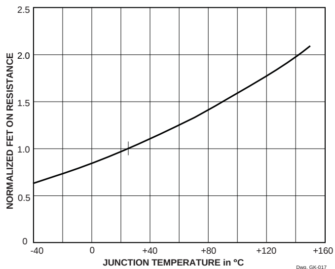
FIGURE 8. NORMALIZED ON RESISTANCE vs TEMPERATURE
