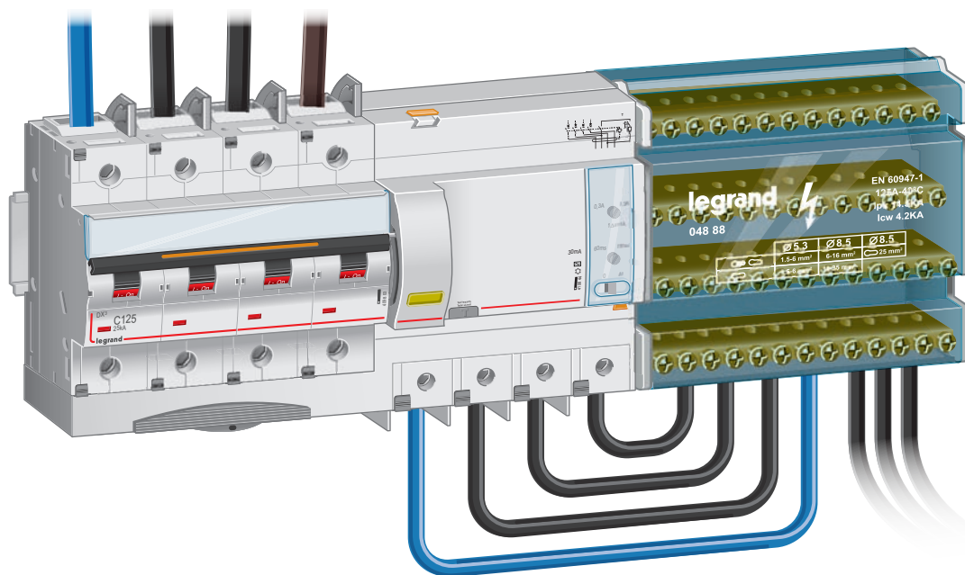
125 A four pole modular distribution block: ideal for distribution at the supply end of secondary boards
