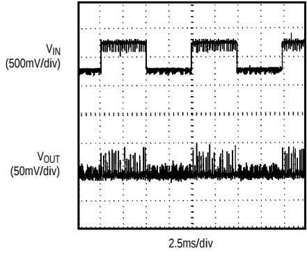
LINE-TRANSIENT RESPONSE
