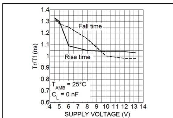
FIGURE 2-10: Rise and Fall Time vs. Supply Voltage.
