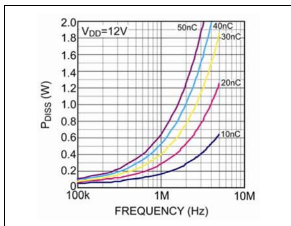
FIGURE 5-4: Driver Power Dissipation.
