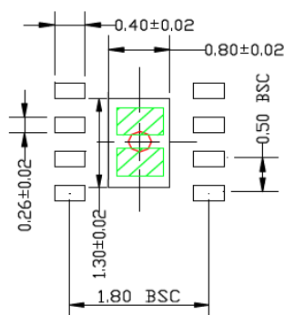
RECOMMENDED LAND PATTERN NOTE: 4, 5
