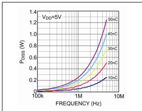
FIGURE 5-3: Driver Power Dissipation.
