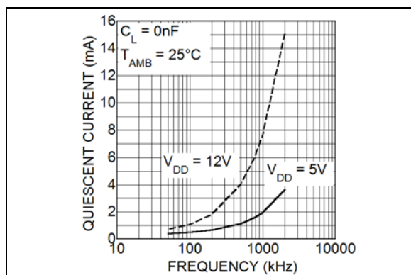
FIGURE 2-8: Quiescent Current vs. Frequency.
