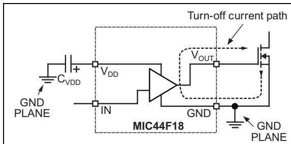
FIGURE 5-7: Critical Current Paths for High Driver Outputs.
