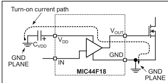
FIGURE 5-6: Critical Current Paths for High Driver Outputs.
