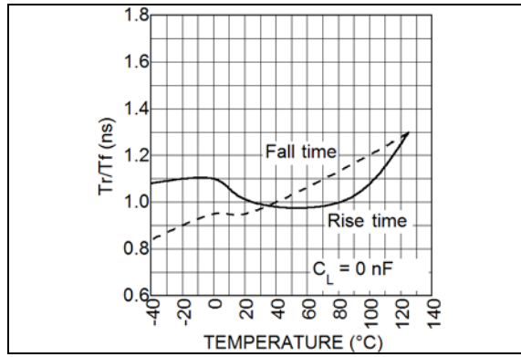
FIGURE 2-12: Rise and Fall Time (12V) vs. Temperature.
