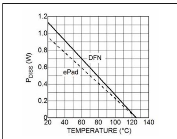
FIGURE 5-5: Maximum Driver Power Dissipation.
