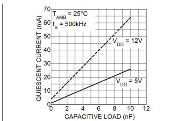
FIGURE 2-9: Quiescent Current vs. Capacitive Load.
