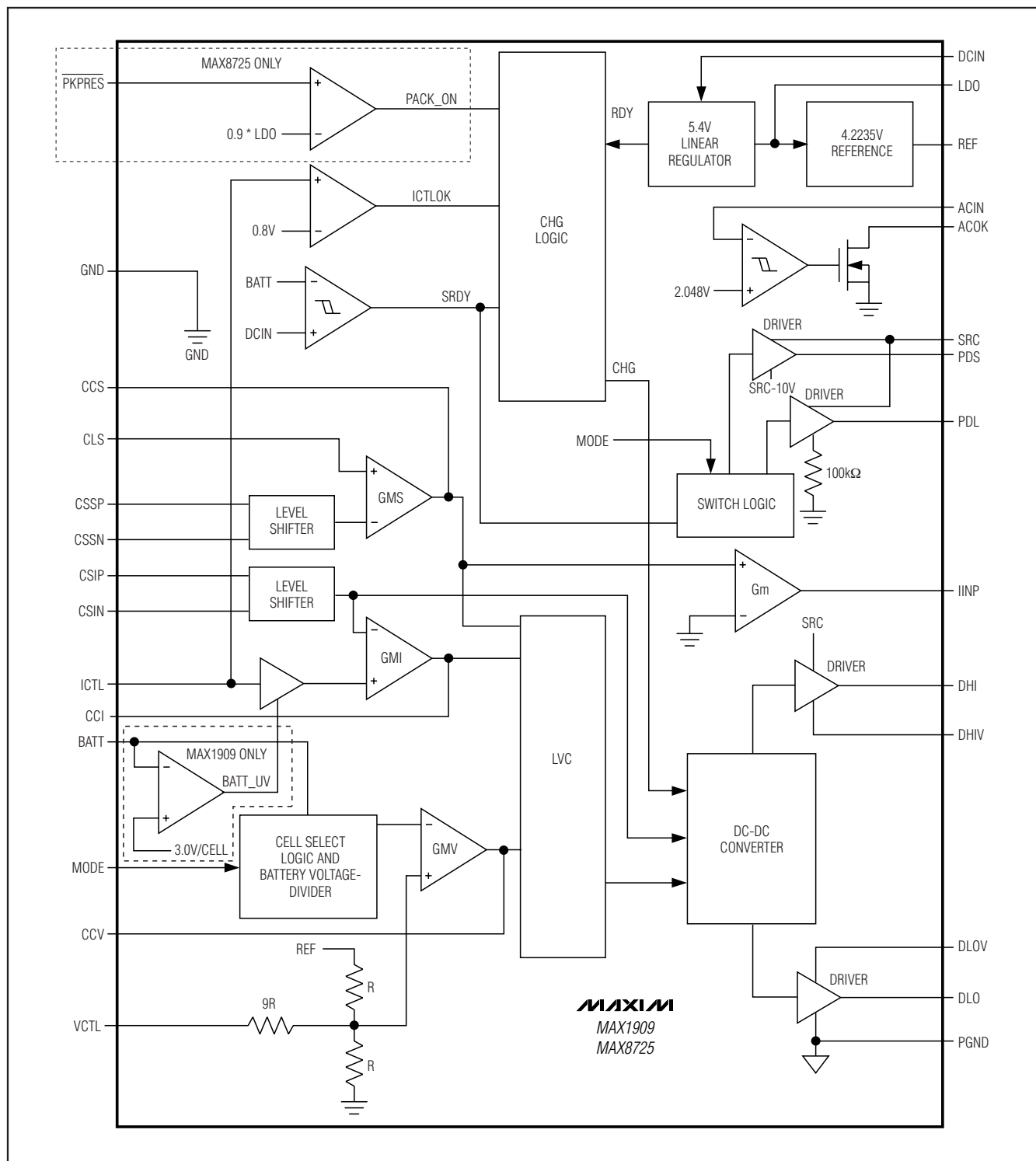
Figure 3. Functional Diagram
