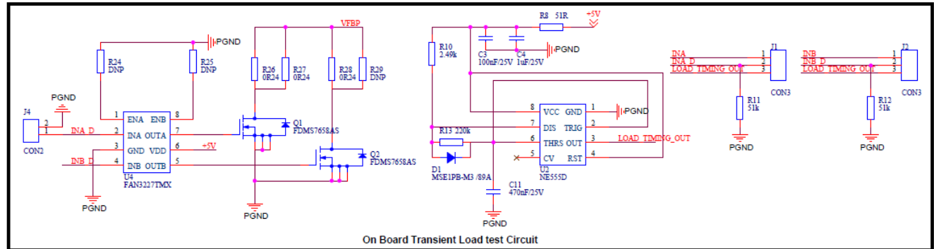
On Board Transient Load test Circuit
