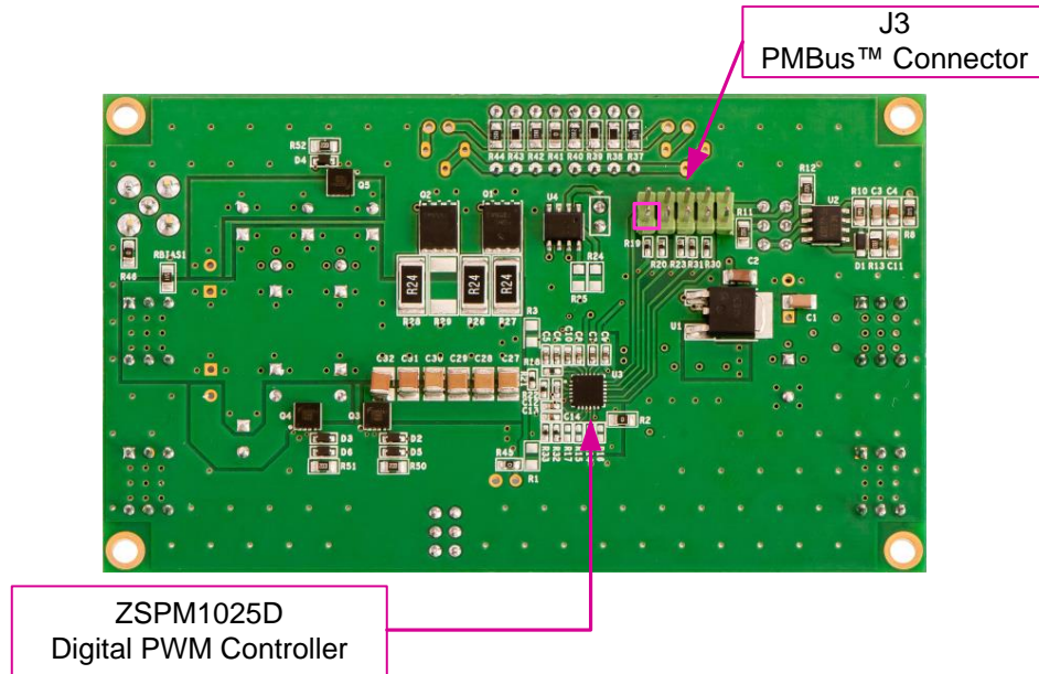
Figure 2.2 ZSPM8825-KIT Evaluation Board (Bottom Side)
