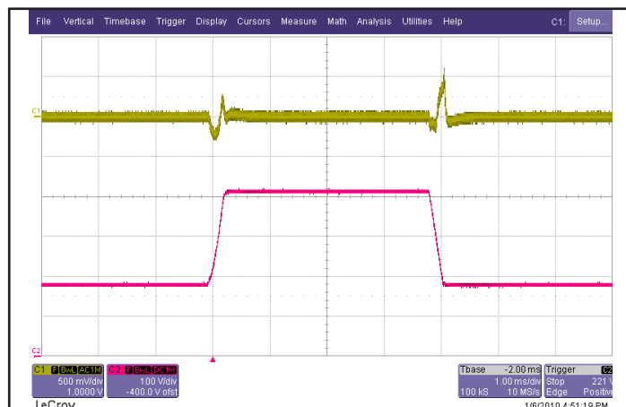
Figure 6: Output voltage response to step-change in input voltage (180V - 425V - 180V), at 25A load current. Load cap: 15μF tantalum capacitor and 1μF ceramic cap. Ch 1: V out (500mV/div), Ch 2: V in (100V/div).
