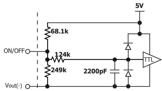
Figure B: Internal ON/OFF pin circuitry
