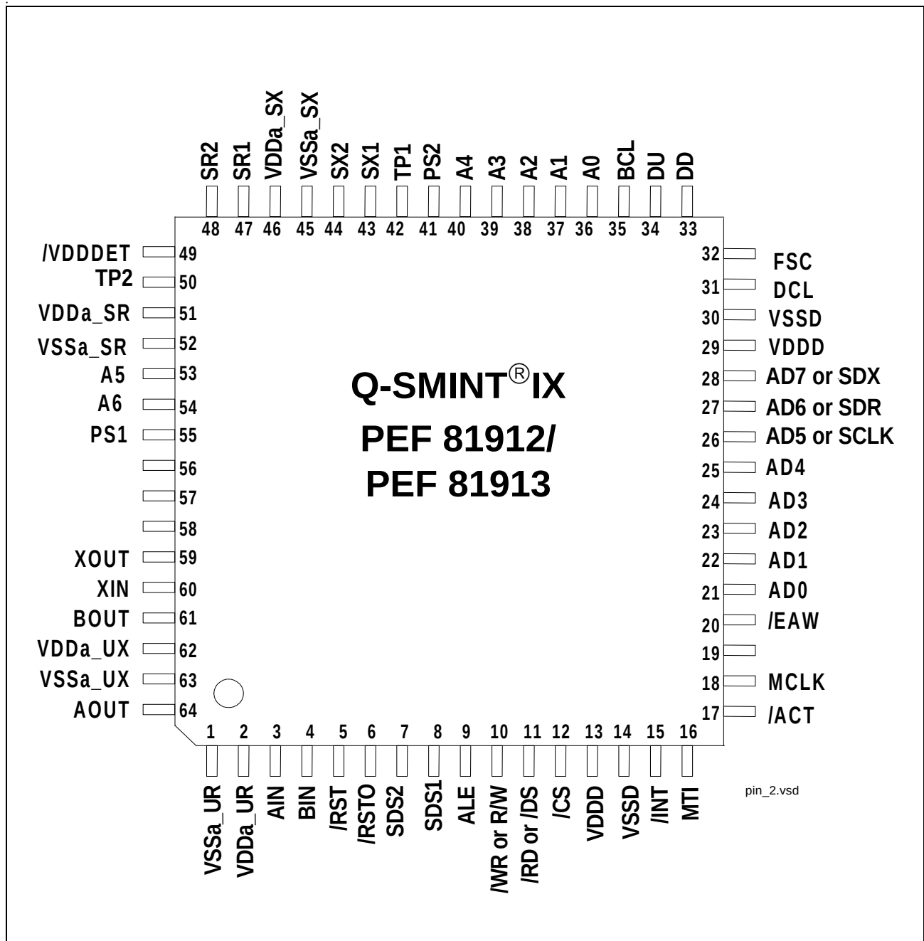
Figure 1 Pin Configuration
