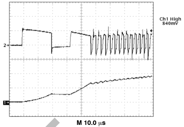
Figure 6. CS5151 Demonstration Board Enable Startup Waveforms
