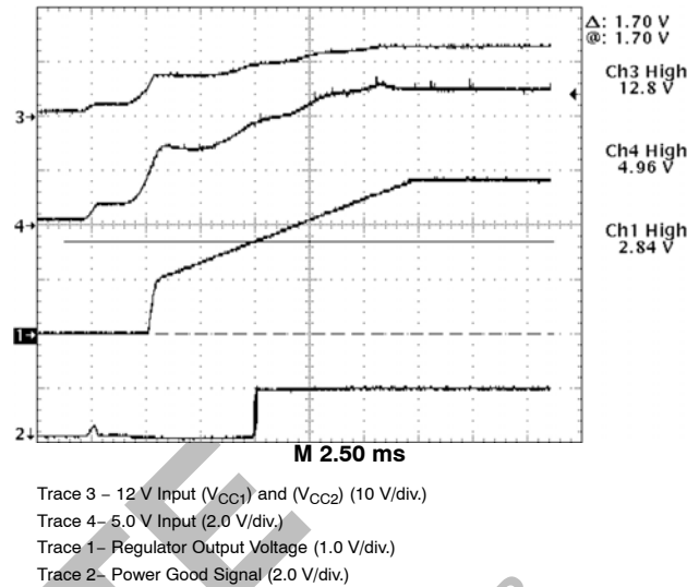
Figure 16. CS5151 Demonstration Board During Power Up. Power Good Signal is Activated when Output Voltage Reaches 1.70 V.
