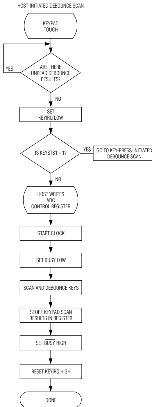
Figure 26. Host-Initiated Debounce Scan
