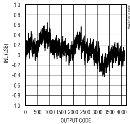
ADC INTEGRAL NONLINEARITY vs. OUTPUT CODE
