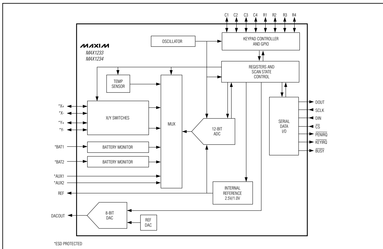
Figure 1. Block Diagram
