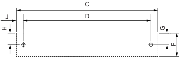
MOUNTING DETAIL
