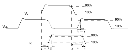
Figure 30. Switching waveform
