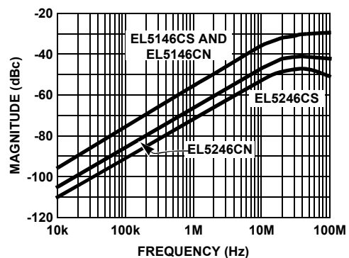
FIGURE 44. OFF ISOLATION - EL5146 AND EL5246
