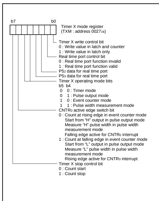
Fig. 22 Structure of timer X mode register
