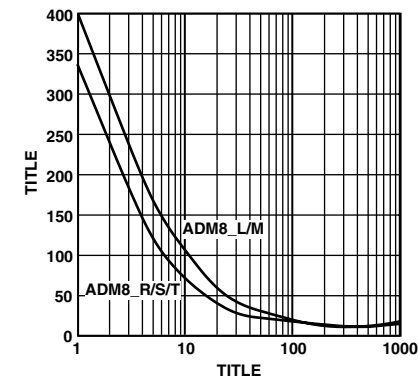
TPC 2. Maximum Transient Duration Without Causing a RESET Pulse vs. RESET Comparator Overdrive
