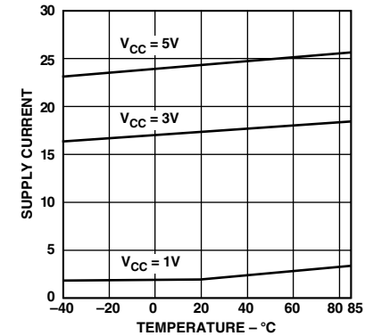
TPC 1. Supply Current vs. Temperature (No Load)
