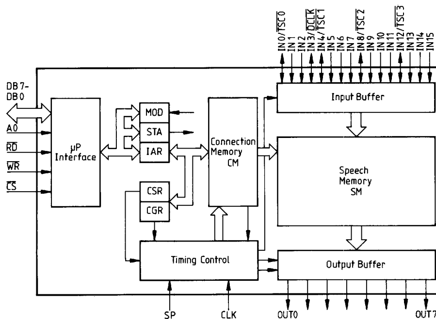
Block Diagram of the PEx 2045
