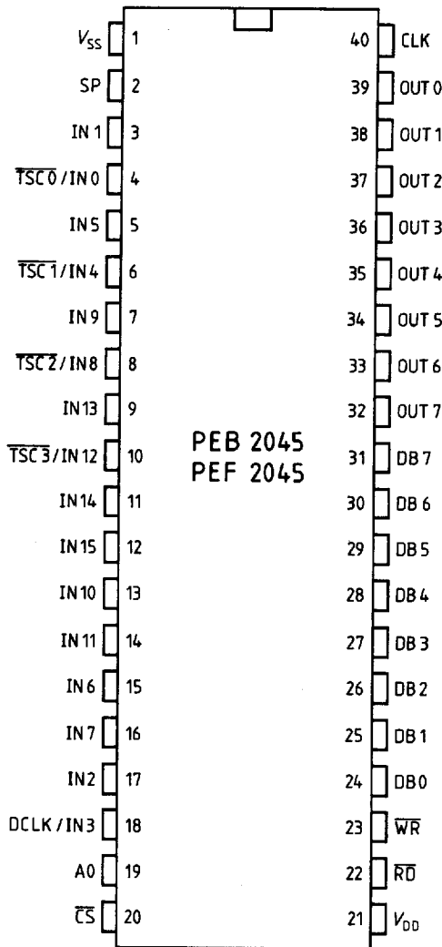
P-DIP-40 C-DIP-40
