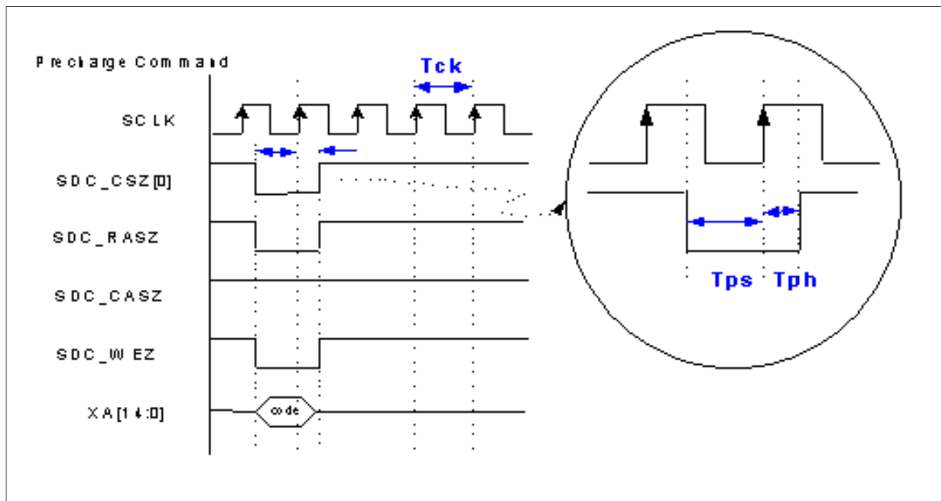
Figure 17 Precharge Command
