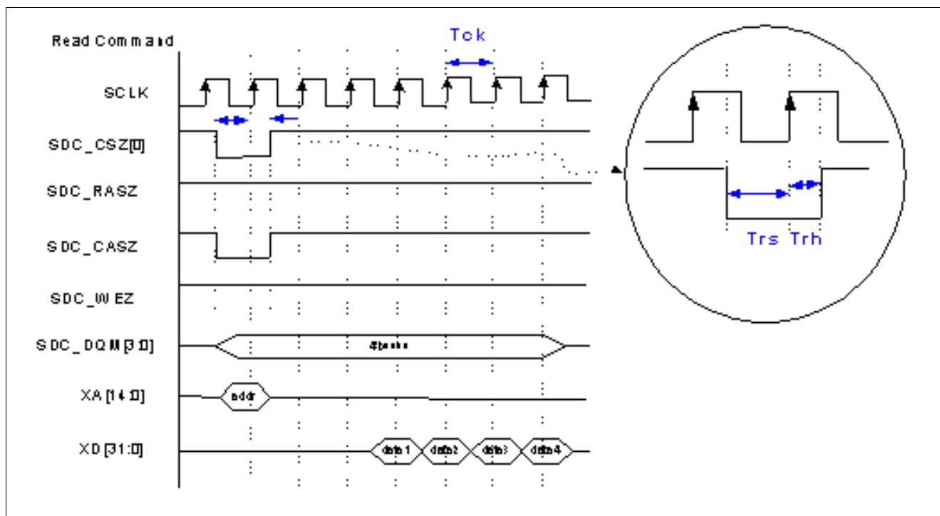
Figure 20 Read Command
