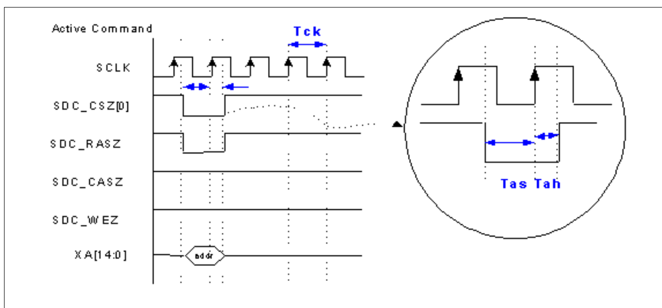
Figure 18 Active Command
