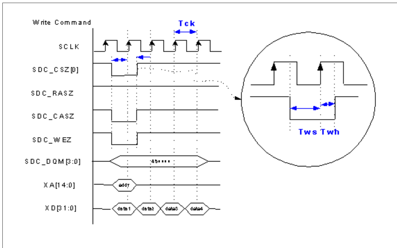
Figure 19 Write Command
