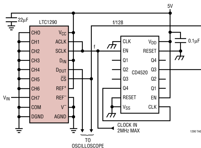
A “Quick Look” Circuit for the LTC1290
