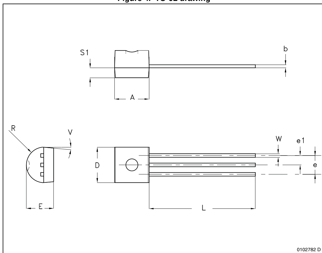
Figure 4. TO-92 drawing
